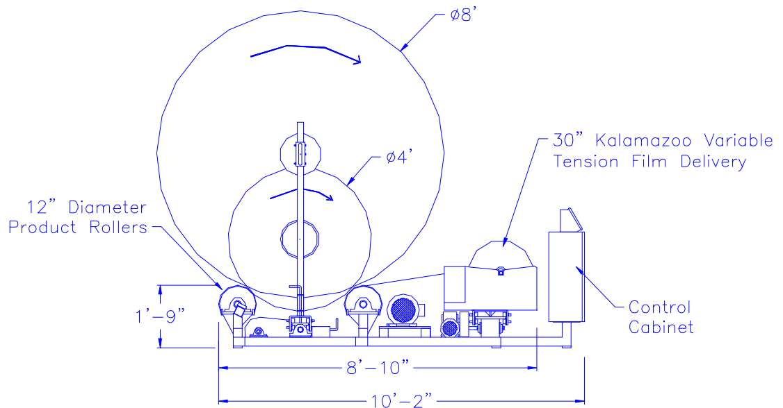
SIDE VIEW
